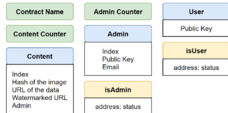
Fig. 2. Class diagram of the smart contract
