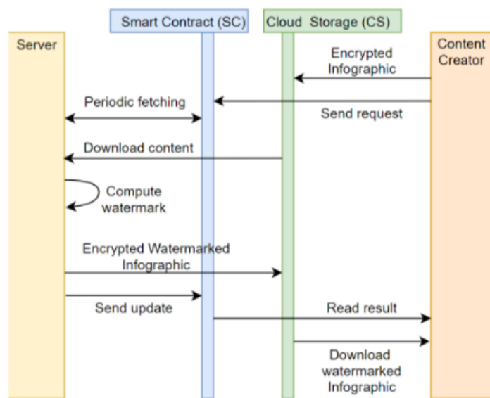
Fig. 3. Sequence diagram of the infographic watermarking request
