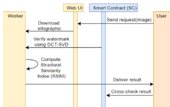
Fig. 4. Sequence diagram of the infographic validation using two-factor verification
