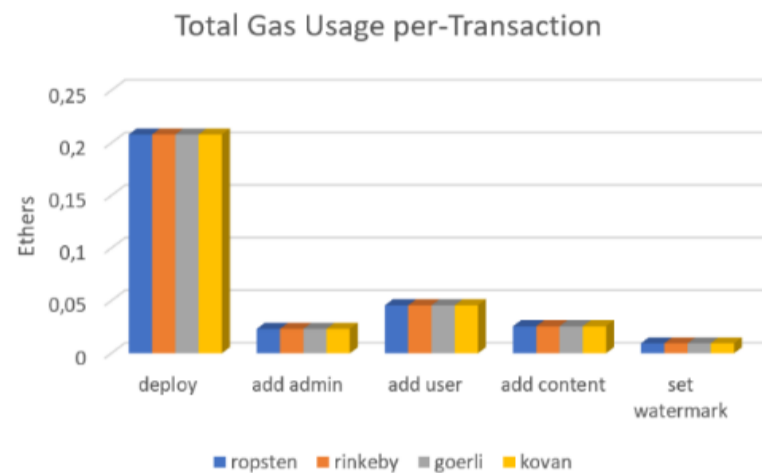
Fig. 7. Comparison of Total gas usage by the Test Networks
