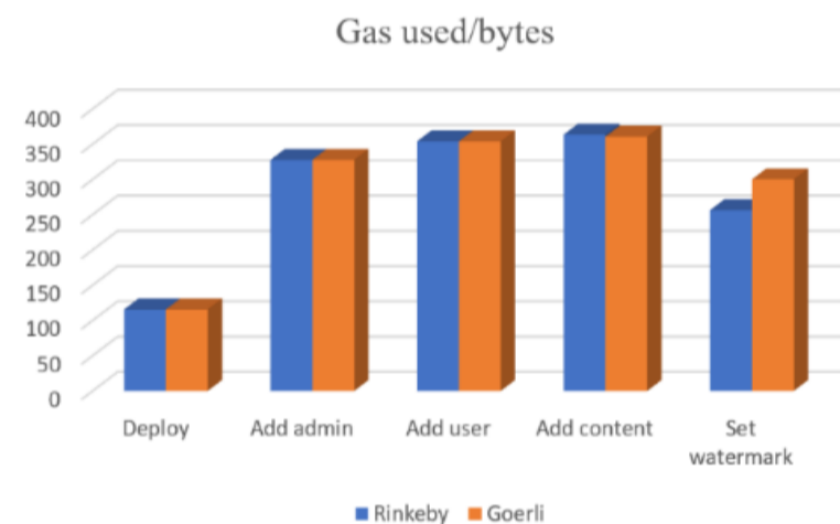
Fig. 8. Gas usage over different data value
