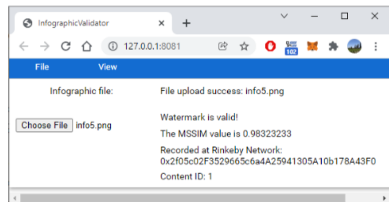
Fig. 6. Web-based validation for infographic and its result.
