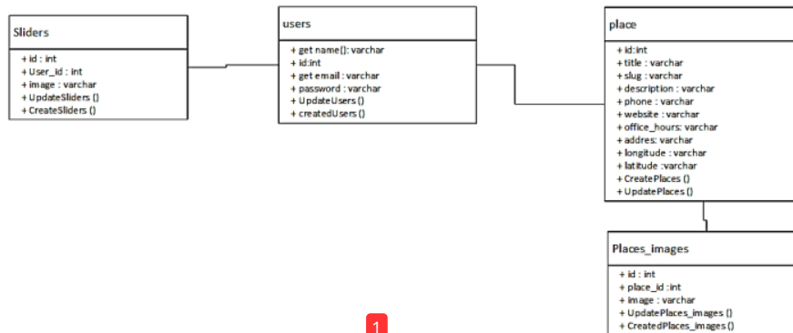
Gambar 8. Class Diagram
