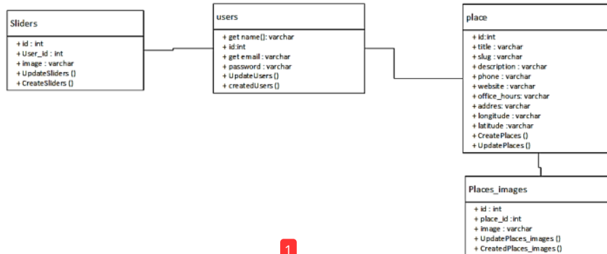
Gambar 8. Class Diagram
