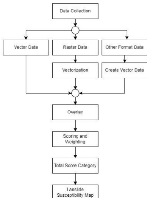
Figure 1. Research Flow
