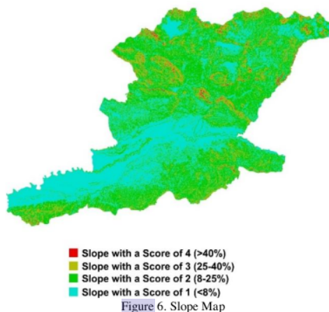
Figure 6. Slope Map
