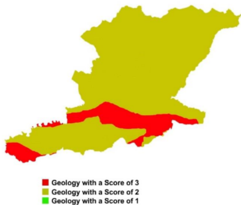
Figure 4. Geological Map
