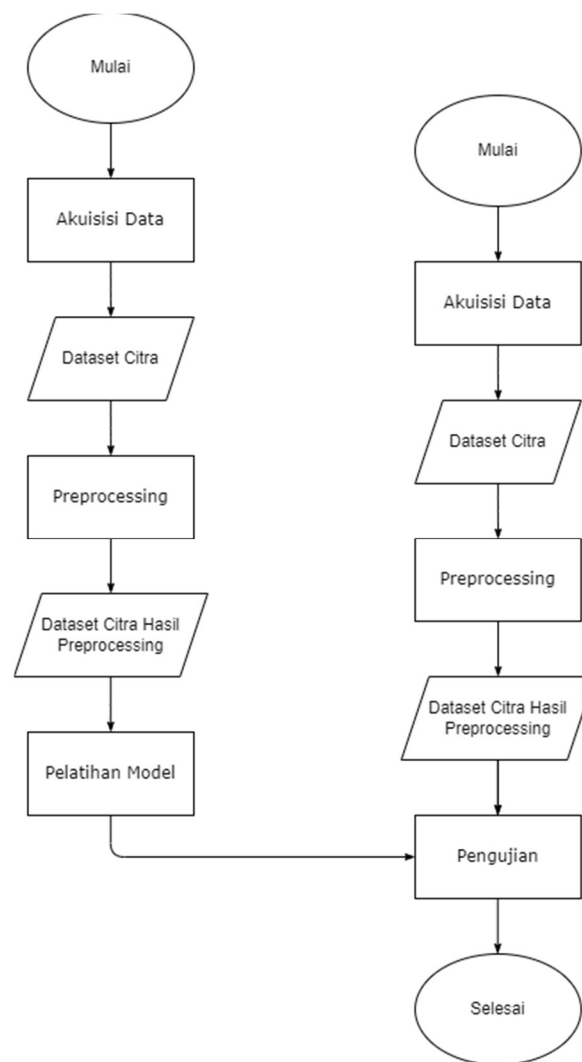
Gambar 8. Diagram Sistem Proses (a) Training (b) Testing
