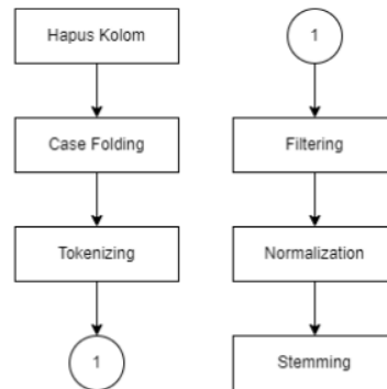
Gbr 3. Tahapan preprocessing
