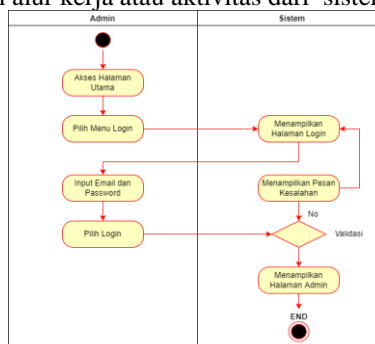
Gambar 3. Diagram Activity Login Admin
