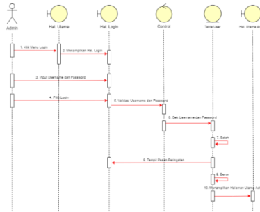
Gambar 4. Diagram Sequence Login Admin
