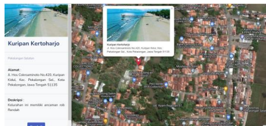
Gambar 14. Halaman Detail
