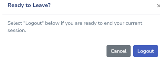
Gambar 12. Logout Admin
