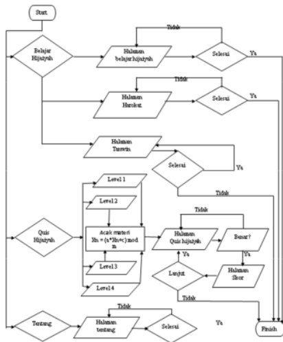
Gambar 3. Flowchart
