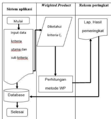
Gambar 2. Flowchart Metode WP
