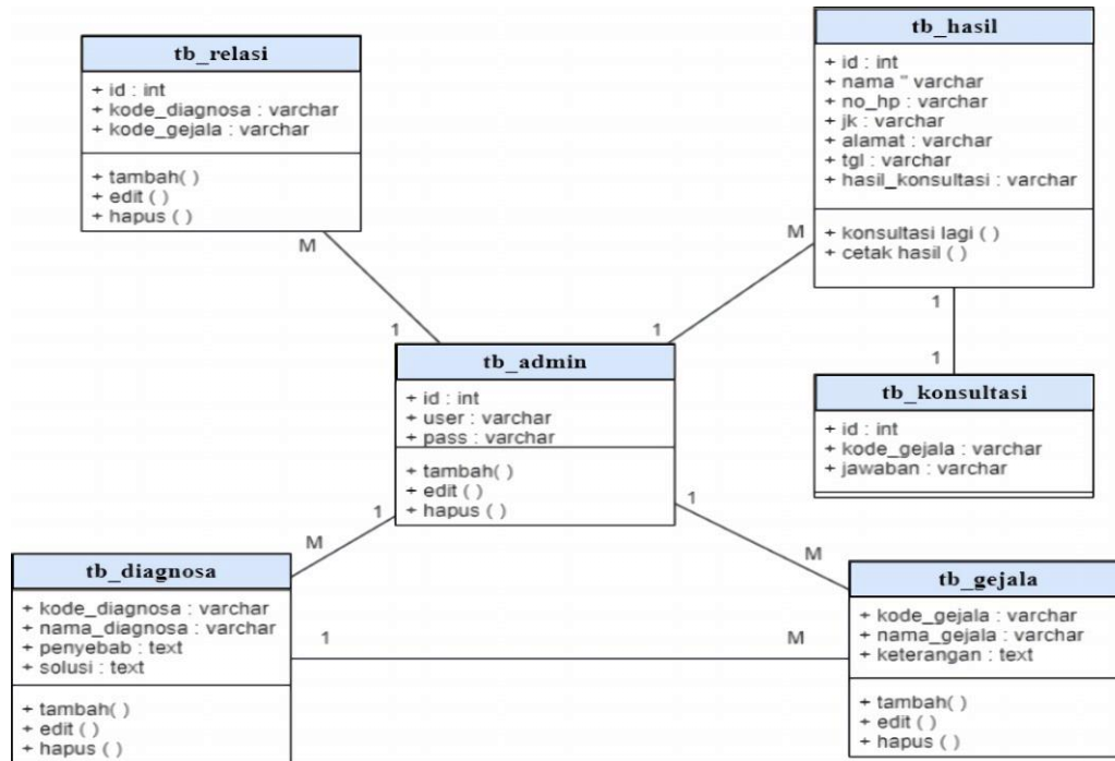
Gambar 5. Class Diagram
