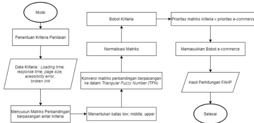
Gambar 4. Diagram Pengolahan Data Fuzzy Analytical Hierarchy Process
