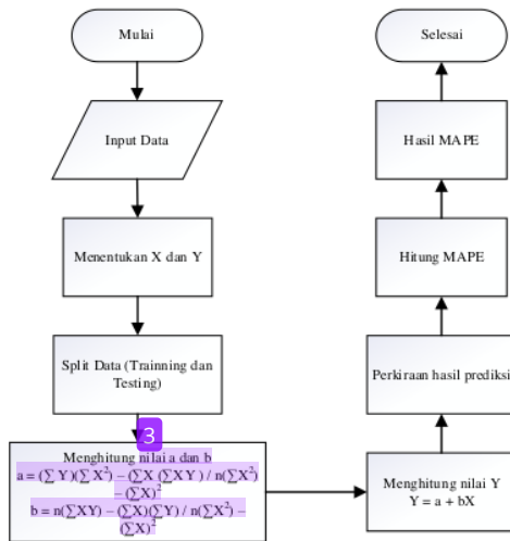
Gambar 6 Flowchart Metode Linear Regression
