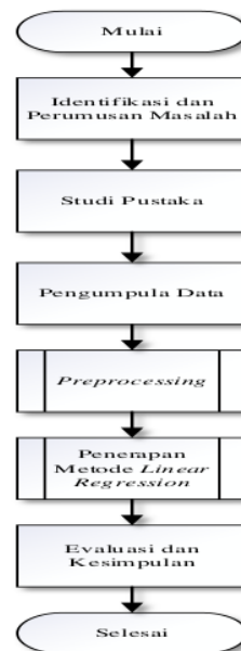
Gambar 3 Flowchart Penelitian
