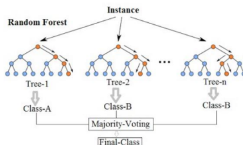
Fig. 5 Random Forest Structure
