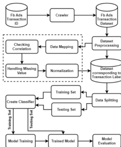
Fig. 6 Our Purposed Methodology
