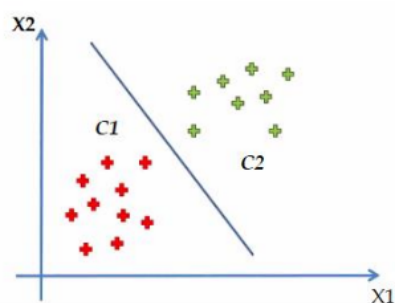
Fig.1 Linearly Separable
