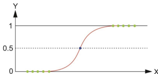
Fig. 3 Logistic Curve Function
