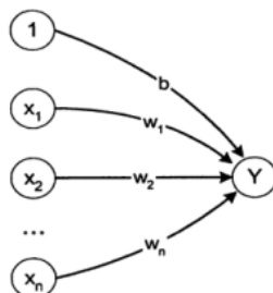
Fig. 2 Perceptron Network Diagram
