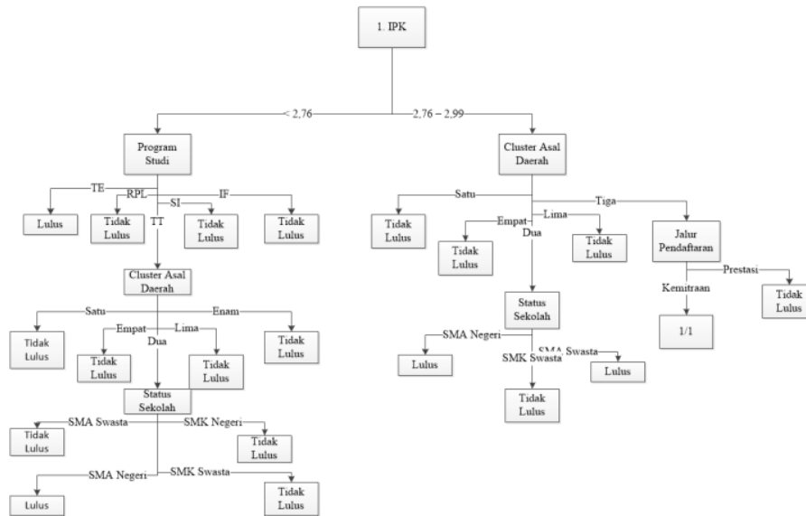
Gambar 2. Decision Tree
