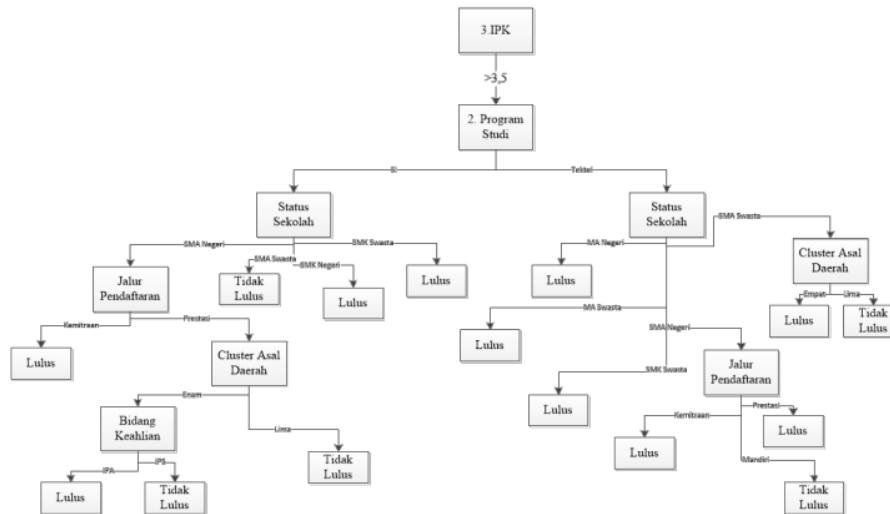
Gambar 7. Decision Tree (Lanjutan)
