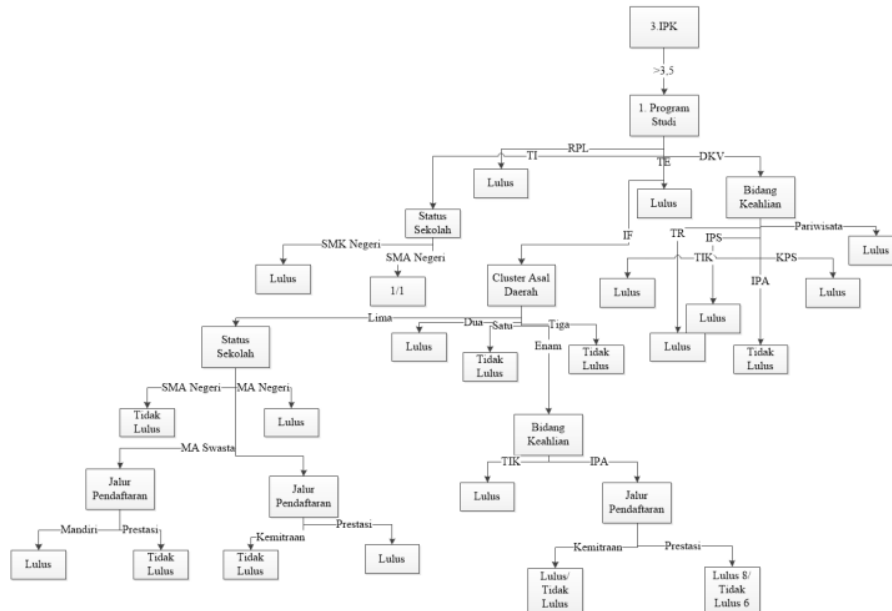
Gambar 6. Decision Tree (Lanjutan)
