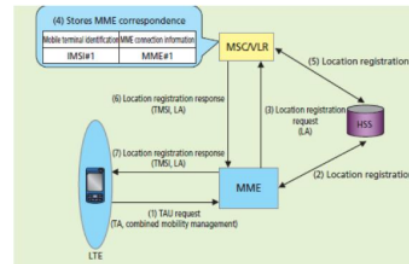
Figure 3: CS Fallback Registration location Procedure [11]
