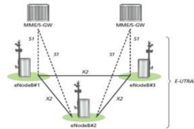
Figure 1: E-UTRAN Architecture [5]
