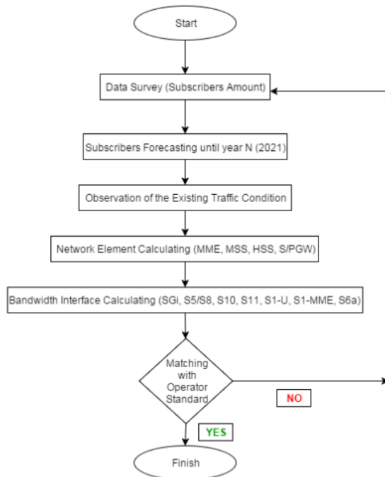
Figure 4: Planning of 4G LTE EPC
