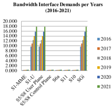
Figure 5: Bandwidth Interface requirement per Years (2016-2021) (Gbps)
