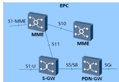
Figure 2: EPC Architecture and The Interfaces [6]
