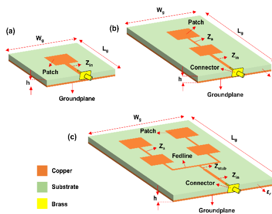
Fig. 1 – Design of the proposed antenna: (a) single element, (b) series array with 2x1 element, (c) planar series array with 2x2 element
