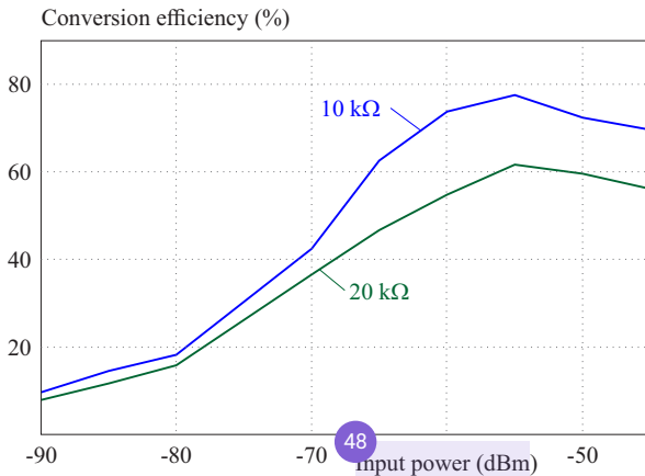
Fig. 18. Conversion efficiency of the proposed rectenna (with antenna array 2 \times 1 )
