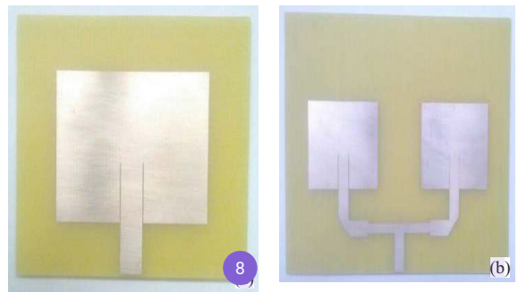
Fig. 6. Photograph of the fabricated antenna (a) single antenna (b) antenna array 2 \times 1
