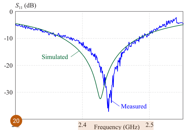
Fig. 7. Return loss of single antenna (simulated & measured)
