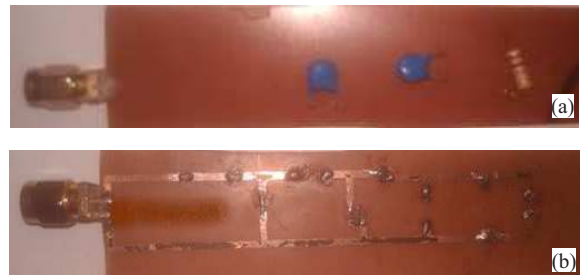
Fig. 15. (a) Front side (b) Backside of fabricated rectifier circuit model A
