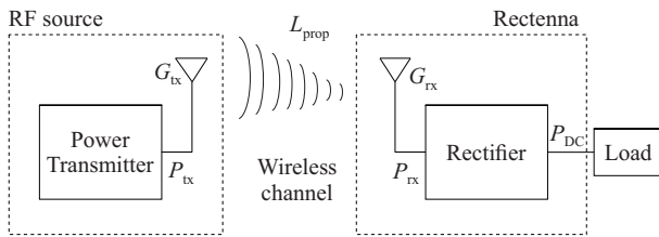
Fig. 1. The basic principle of RF energy harvesting
