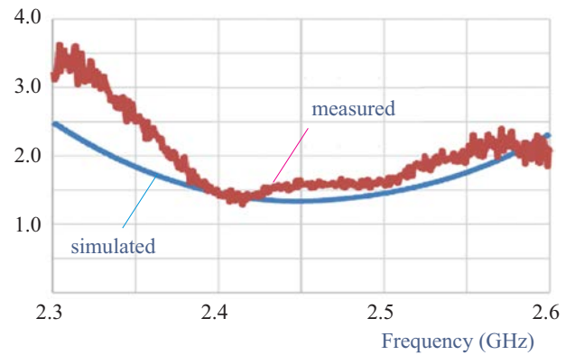
Fig. 12. VSWR of antenna array 2 x 1
