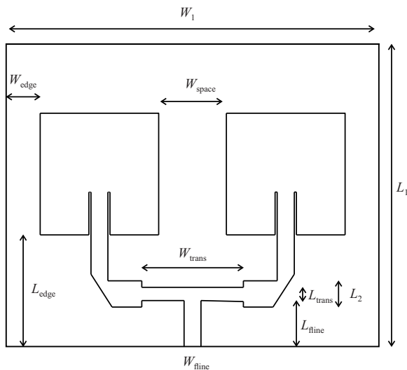
Fig. 5. Configuration of the proposed antenna array 2 \times 1
