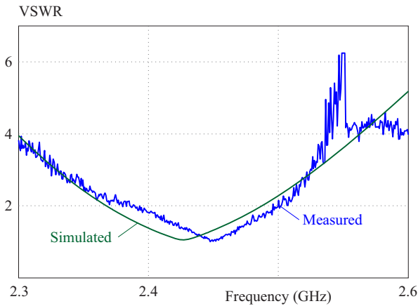
Fig. 9. VSWR of a single antenna (simulated & measured)
