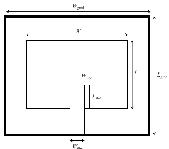
Fig. 3. Geometrical design of a single antenna
