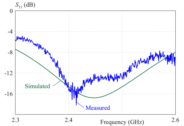
Fig. 10. Return loss performance of antenna array 2 x 1
