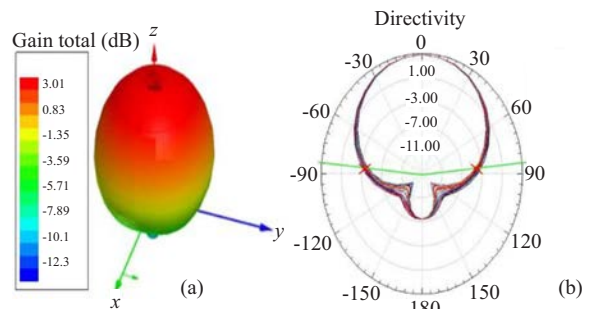
Fig. 8. (a) Gain (b) Radiation pattern of a single antenna (simulated)
