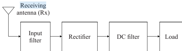
Fig. 2. Basic structure of a rectenna
