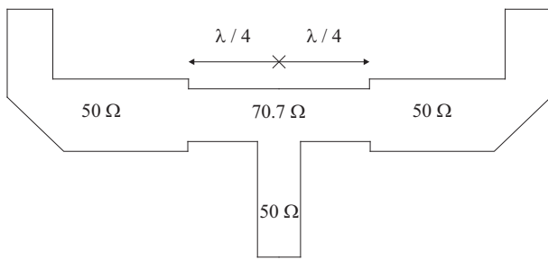
Fig. 4. T-junction
