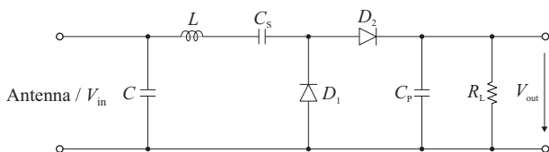
Fig. 16. Schematic configuration of rectifier circuit model B
