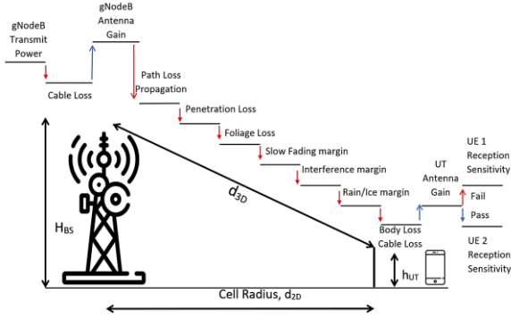
Fig. 8. 5G NR link budget illustration.
