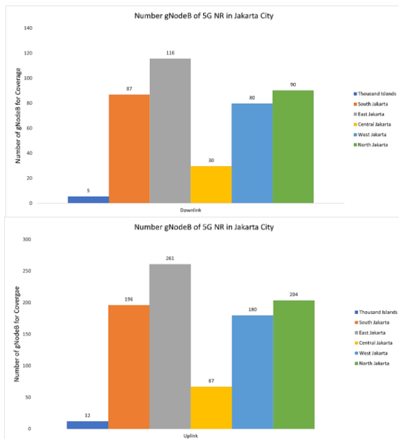
Fig. 13. Coverage uplink and downlink gNodeB.
