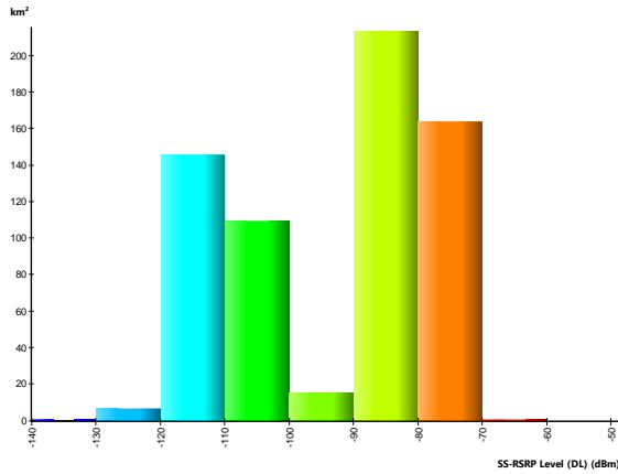
Fig. 16. SS-RSRP network planning results in histogram mode.
