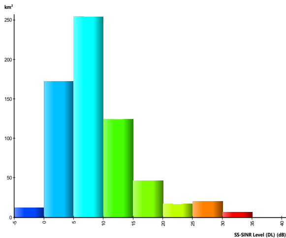
Fig. 18. SS-SINR network planning results in histogram mode.
