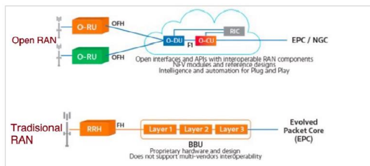
Gambar 1. Arsitektur Open RAN Vs Tradisional RAN Sumber: (Sevinka et al., 2021)
