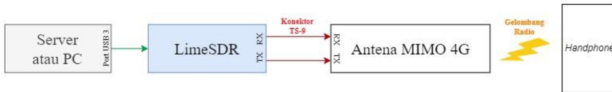
Gambar 5. Rancangan Topologi Jaringan Open RAN 4G
