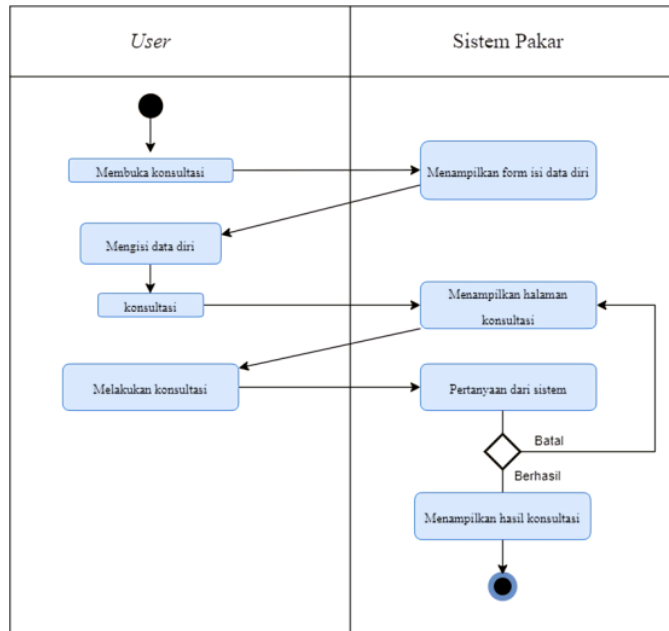
Gambar 3. Activity Diagram
