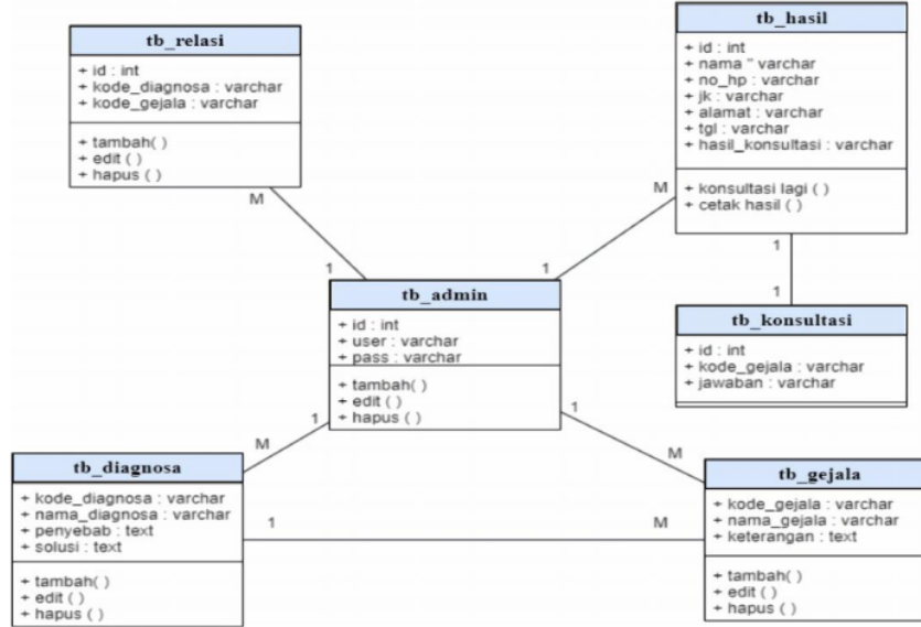
Gambar 5. Class Diagram
