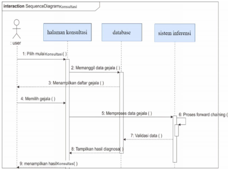
Gambar 4. Sequence Diagram
