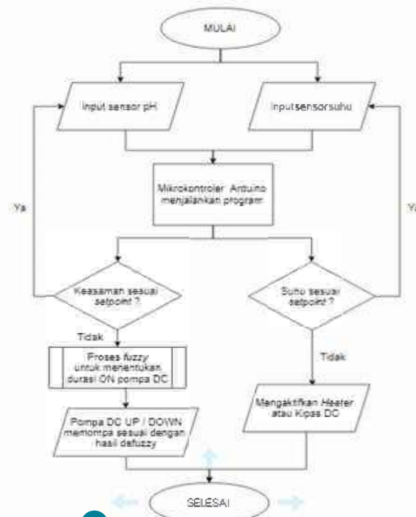
37 Gambar 5 Flowchart Sistem
