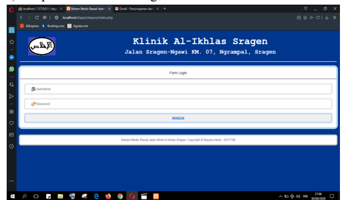
Figure 9. Login Form
