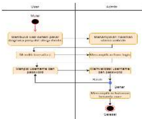
Gambar 1. 3 Activity Diagram.
