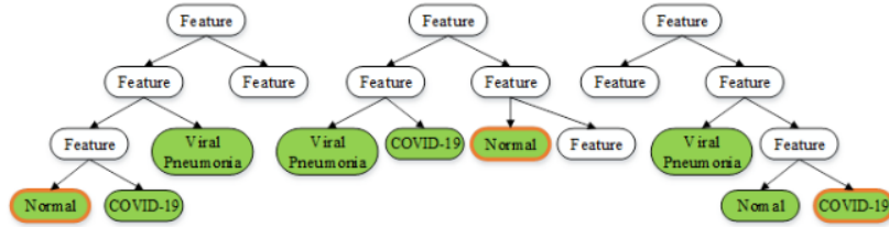
Fig. 5. Illustration of Random Forest method.
