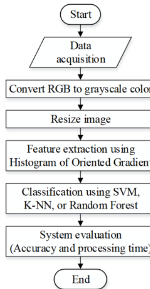
Fig. 1. Steps of research on COVID-19 detection systems.
