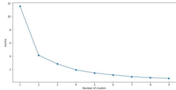
Gambar 6. Elbow Method
