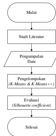
Gambar 1. Flowchart Penelitian
