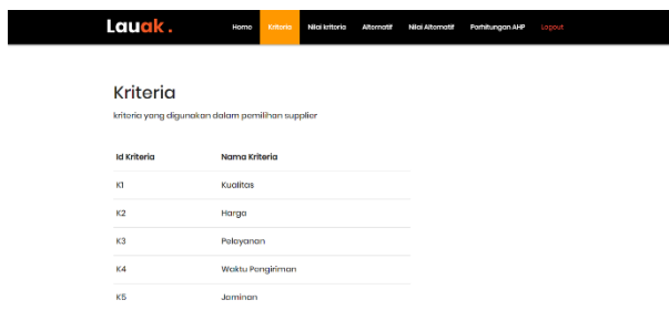
Gambar 4. Kriteria Penilaian
