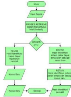
Gambar 2. Flowchart Proses CBR Sistem Pakar
