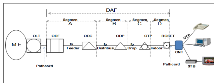
Gambar 2.1 Jaringan FTTH ( Fiber To The Home ) [4]
