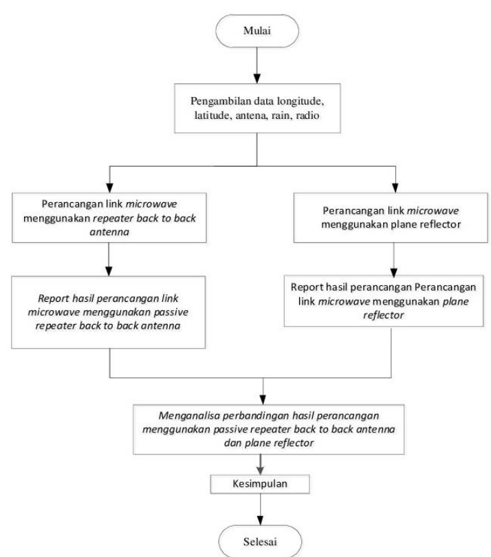
Gambar 3. 2 Flowchart Sistem
