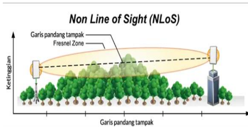
Gambar 3.5 Kondisi Non line of sight [18]
