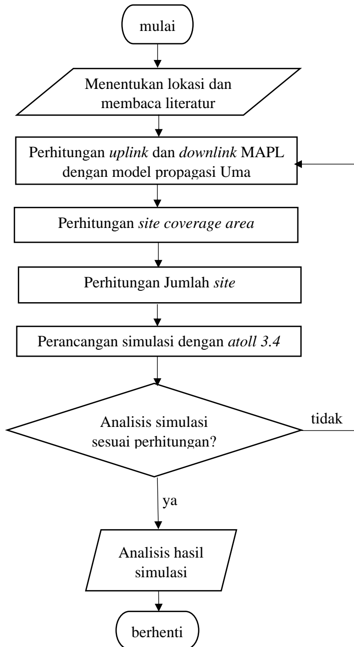
Gambar 3.1 Flowchart penelitian
