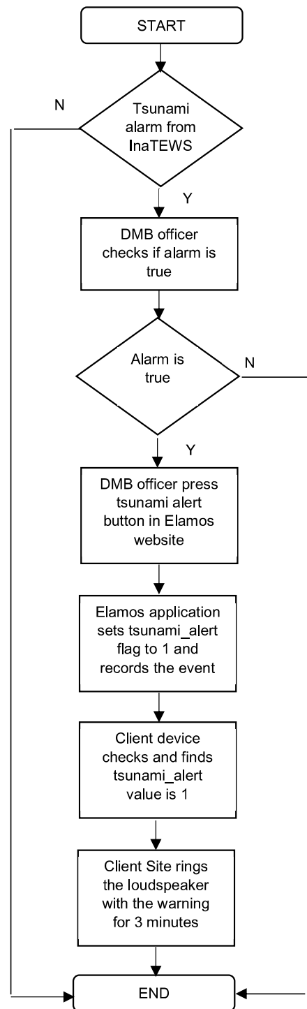
Figure 2. Elamos' application flowchart
