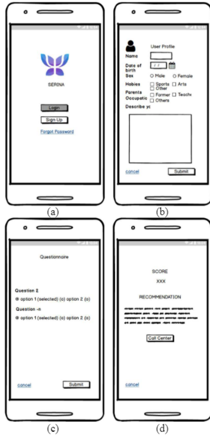
Fig. 3. Low-fidelity design of SERIINA
