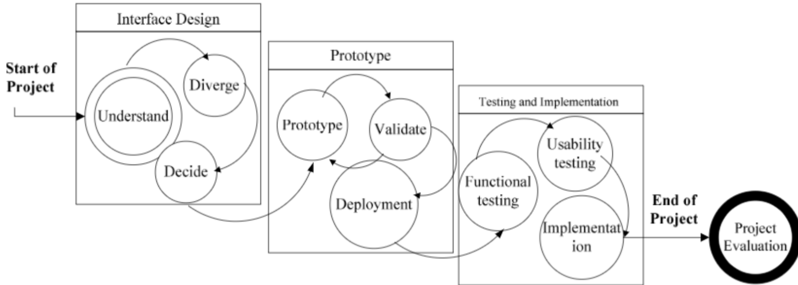
Fig. 1. Extended Rapid Application Development Process
